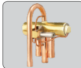
A hot defrost gas valve enables the unit to operate at low ambient temperature.
